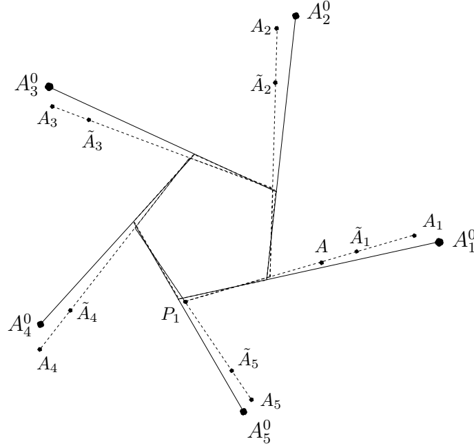
FIGURE 1. Original and perturbed T_k 's.
